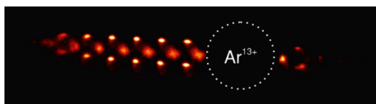
Sympathetically cooled highly-charged ions. Left: \text{Ar}^{13+} in a cloud of laser-cooled \text{Be}^+ ions. Right: Two-ion crystal of a \text{Be}^+ and an \text{Ar}^{13+} ion.
